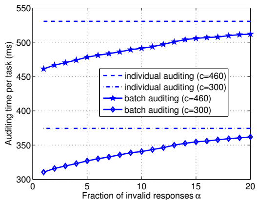
Fig. 3: Comparison on auditing time between batch and individual auditing, when \alpha -fraction of 256 responses are invalid: Per task auditing time denotes the total auditing time divided by the number of tasks.
